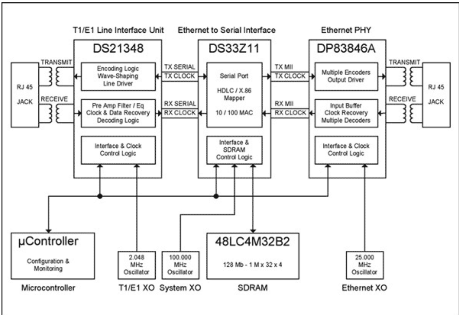
Figure 1. Block Diagram of the Ethernet LAN to Unframed, T1/E1 WAN Bridge
